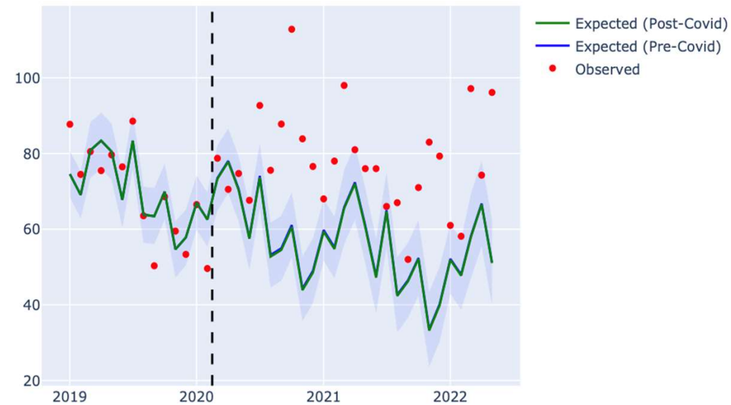
Female (Age: 60-69) Observed Versus Expected Number of Suicides
