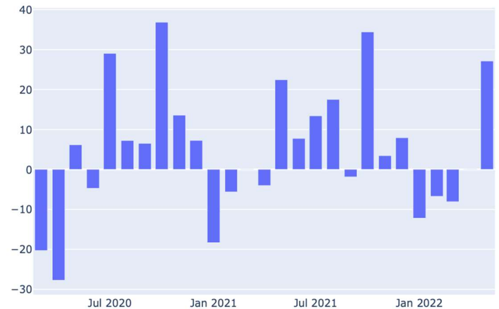
Female (Age: 80-99) Covid-induced Suicides Over Time
