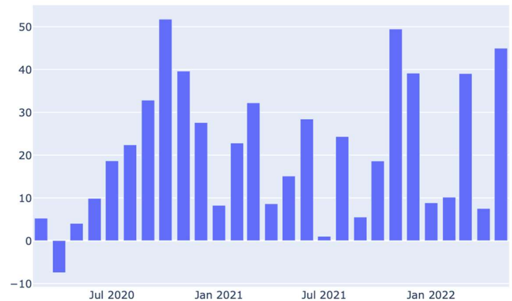
Female (Age: 60-69) Covid-induced Suicides Over Time
